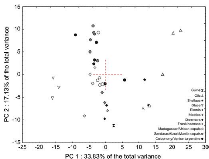
Fig. 4. Score plot of PC1 and PC2. Variables: FT-Raman CH band data points (step=2 cm -1 ), items: 37 reference samples. Some samples are clustered (ex: glues), some are dispersed (ex: pine resins) and some are grouped but among another kind of material (ex: frankincenses within the diterpenic resins).
